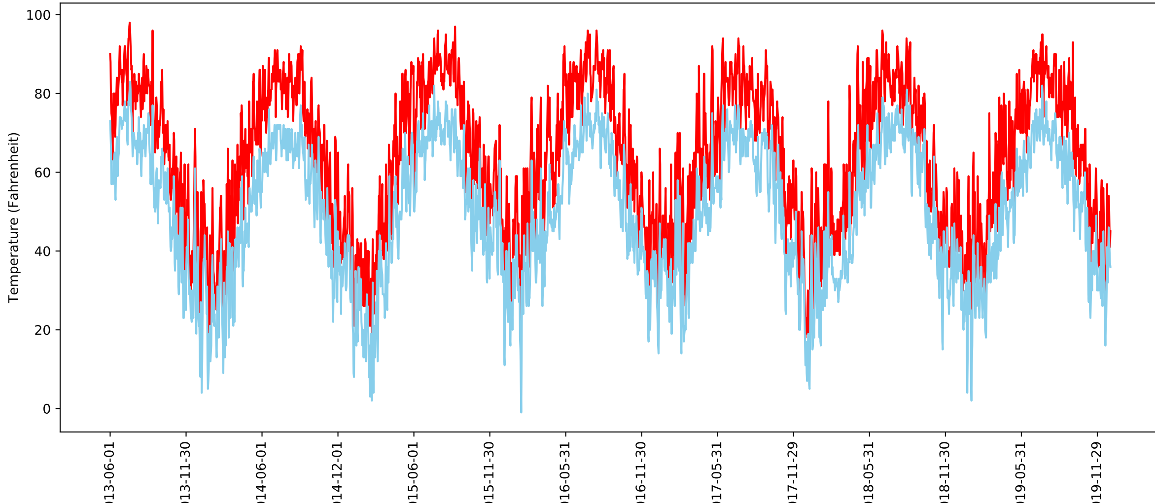
Minimum and maximum temperatures by day
